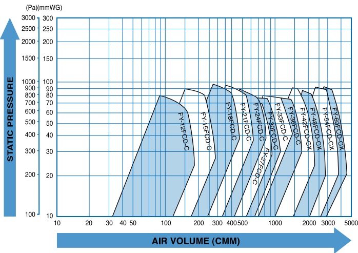
FAN SELECTION CHART (DWDI : DOUBLE-END BEARING, DOUBLE SUCTION TYPE)
